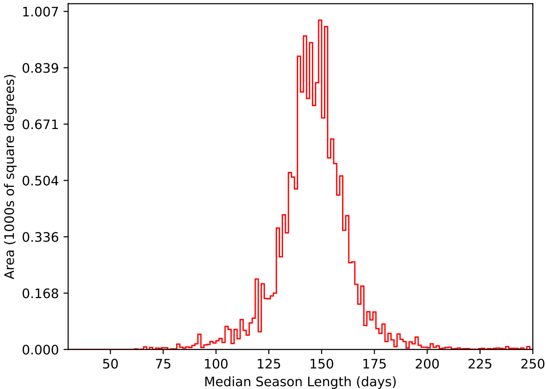
ddf_acor_sf10_lsf15_lsr10_v3.4_10yrs WFD i band: Median Season Length
