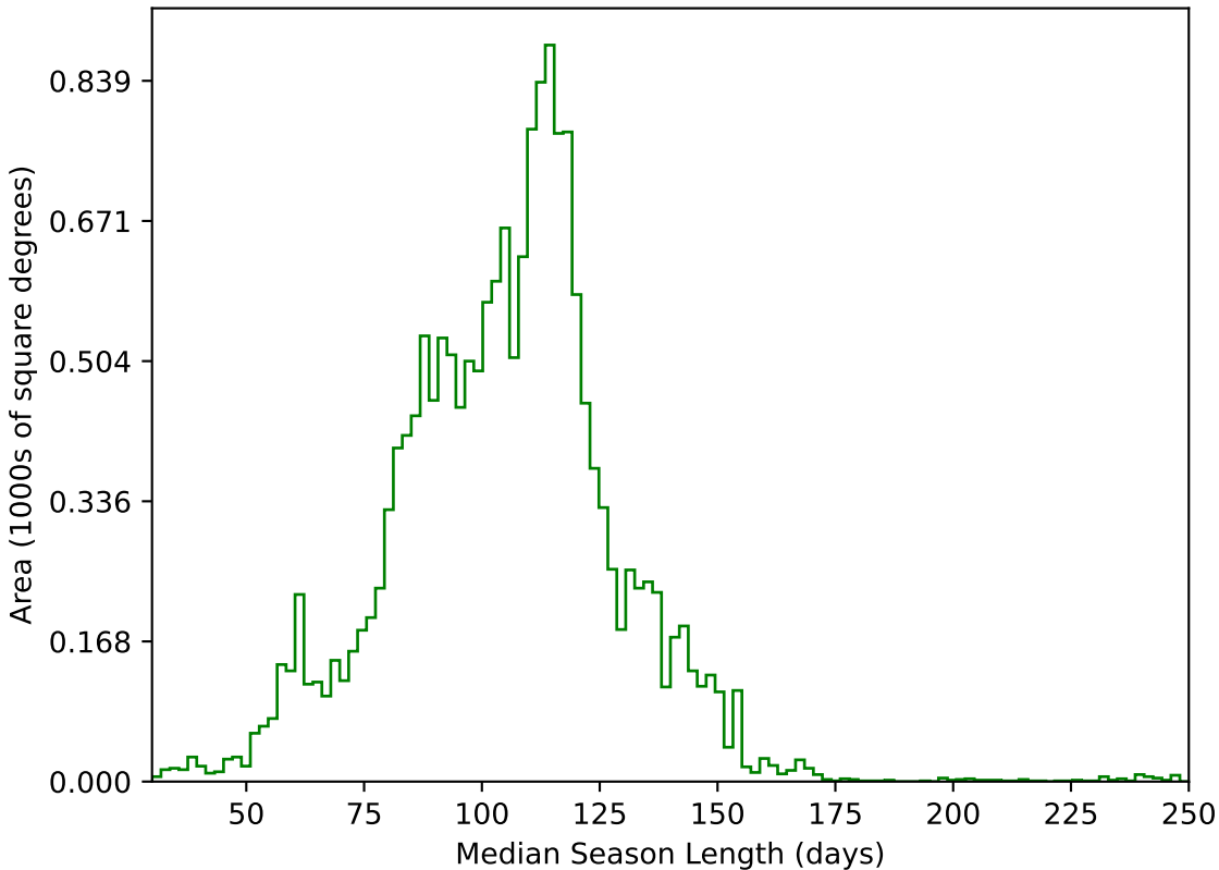
ddf_acor_sf10_ls15_lsr10_v3.4_10yrs WFD g band: Median Season Length
