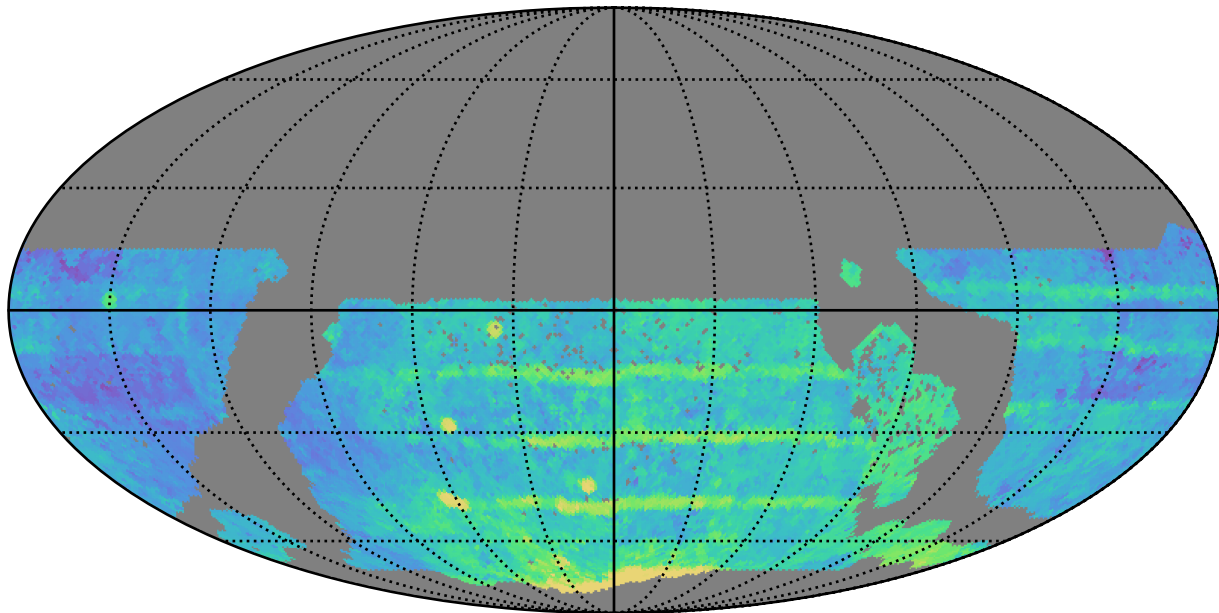
ddf_acor_sf10_lsf15_lsr10_v3.4_10yrs WFD all bands: Median Season Length
