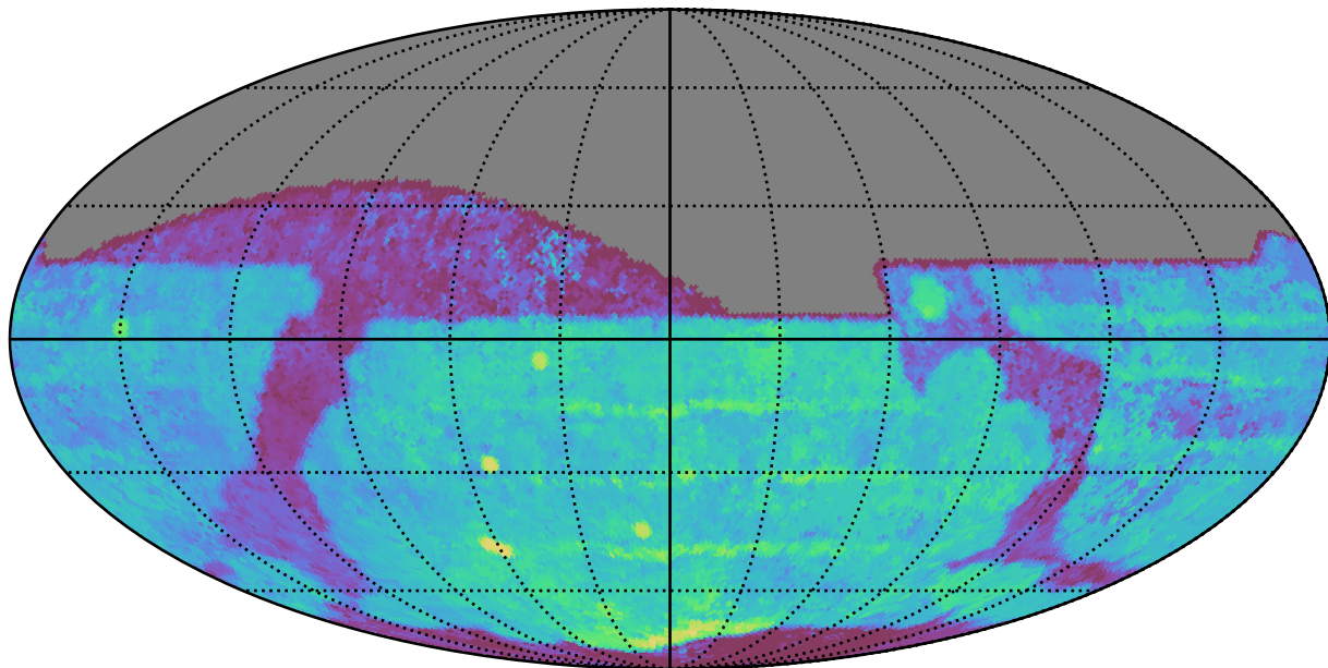
ddf_acor_sf10_lsf15_lsr10_v3.4_10yrs All sky z band: Median Season Length
