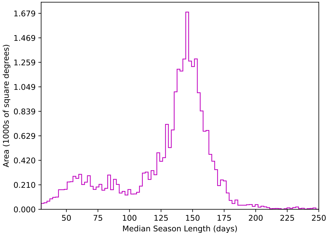
ddf_acor_sf10_lsf15_lsr10_v3.4_10yrs All sky z band: Median Season Length
