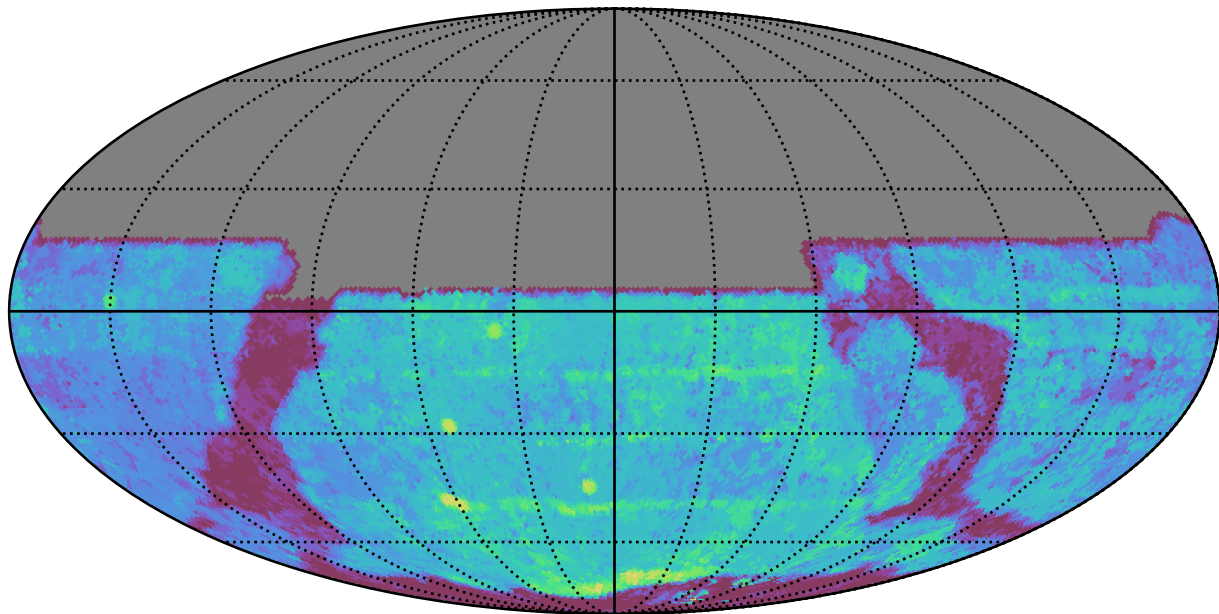
ddf_acor_sf10_ls15_lsr10_v3.4_10yrs All sky y band: Median Season Length
