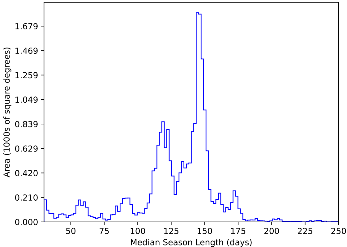
ddf_acor_sf10_lsf15_lsr10_v3.4_10yrs All sky y band: Median Season Length
