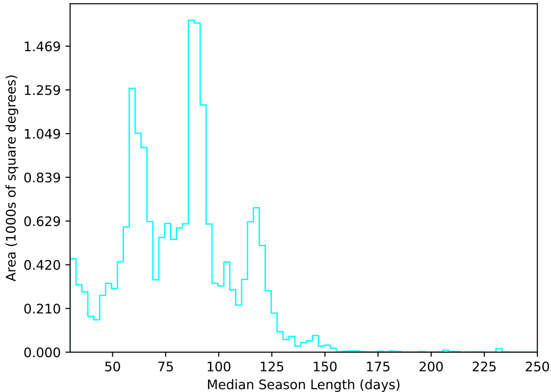
ddf_acor_sf10_lsf15_lsr10_v3.4_10yrs All sky u band: Median Season Length
