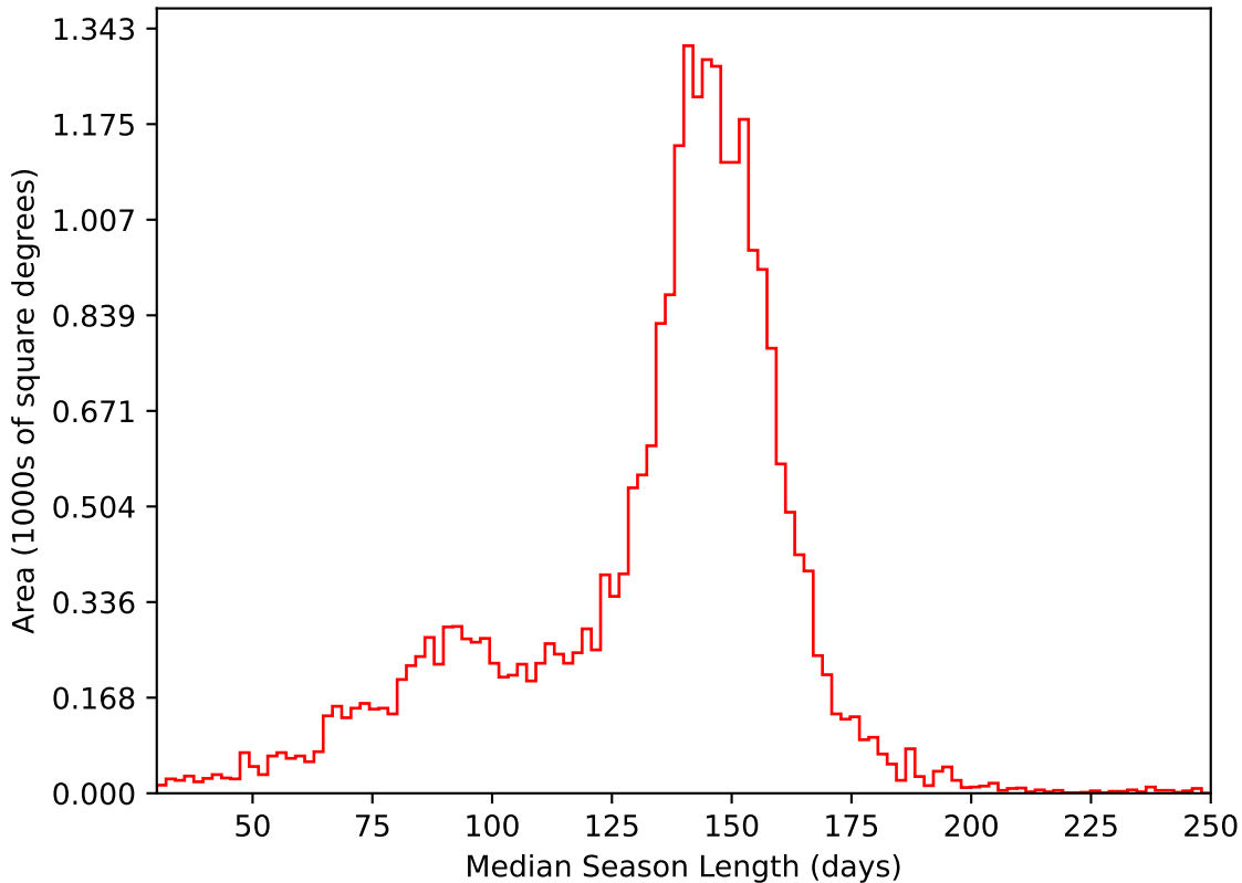
ddf_acor_sf10_lsf15_lsr10_v3.4_10yrs All sky i band: Median Season Length
