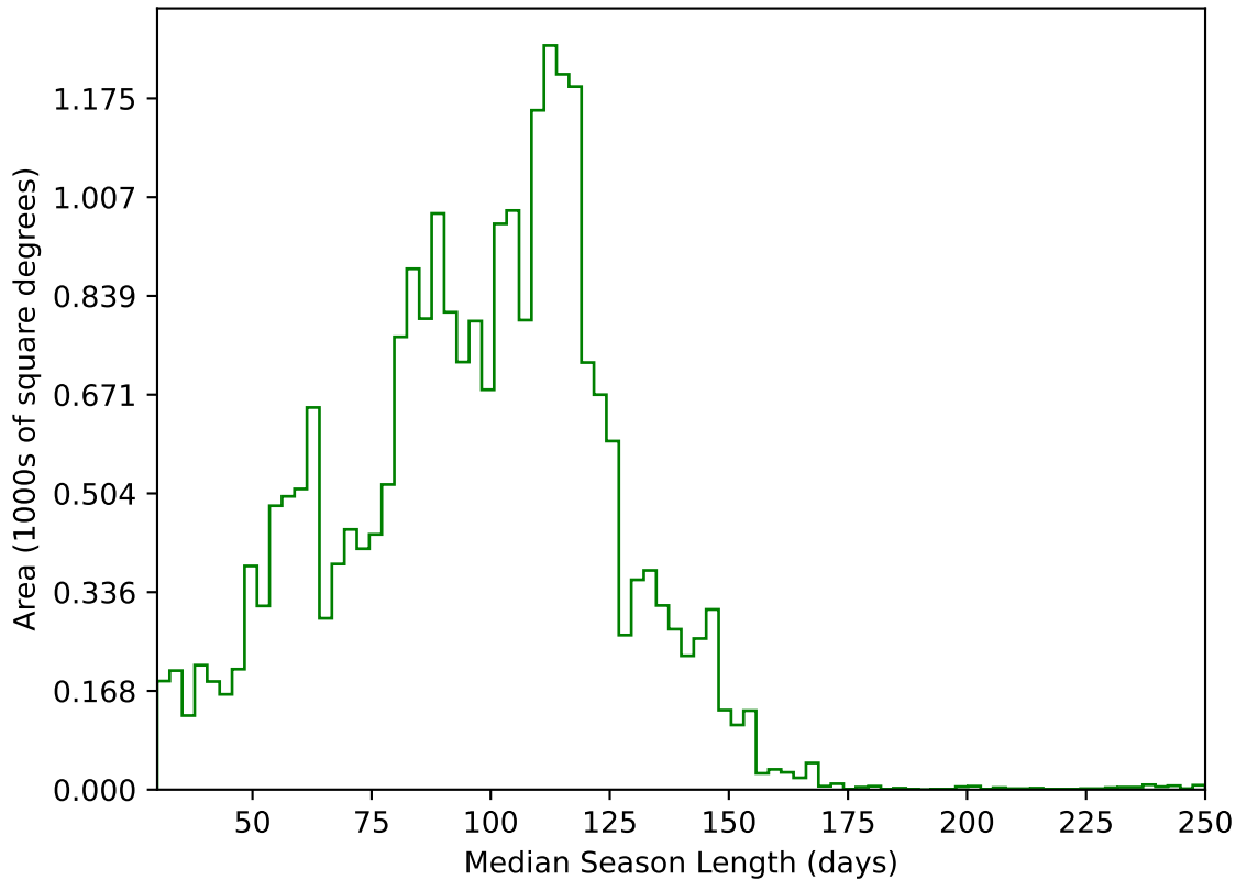
ddf_acor_sf10_lsf15_lsr10_v3.4_10yrs All sky g band: Median Season Length
