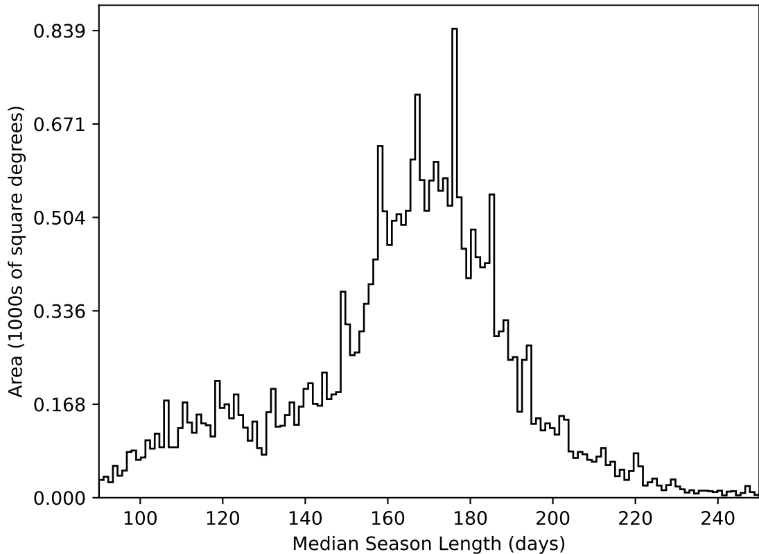
ddf_acor_sf10_lsf15_lsr10_v3.4_10yrs All sky all bands: Median Season Length
