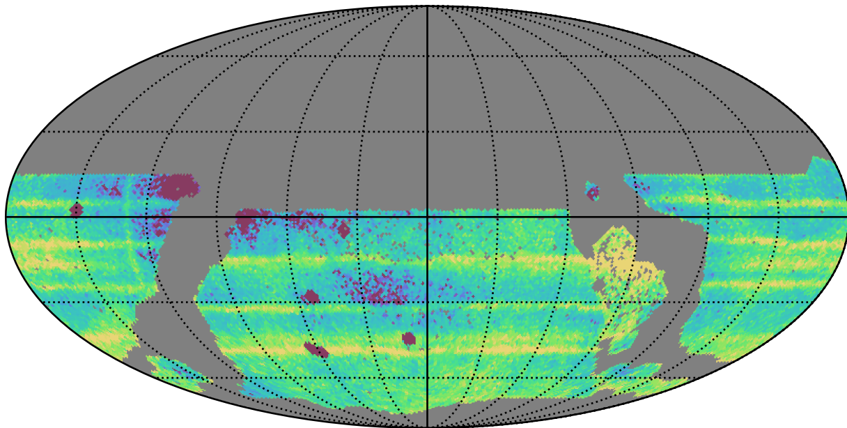
ddf_acor_sf10_lsf15_lsr10_v3.4_10yrs WFD: Median Intra-Night Gap
