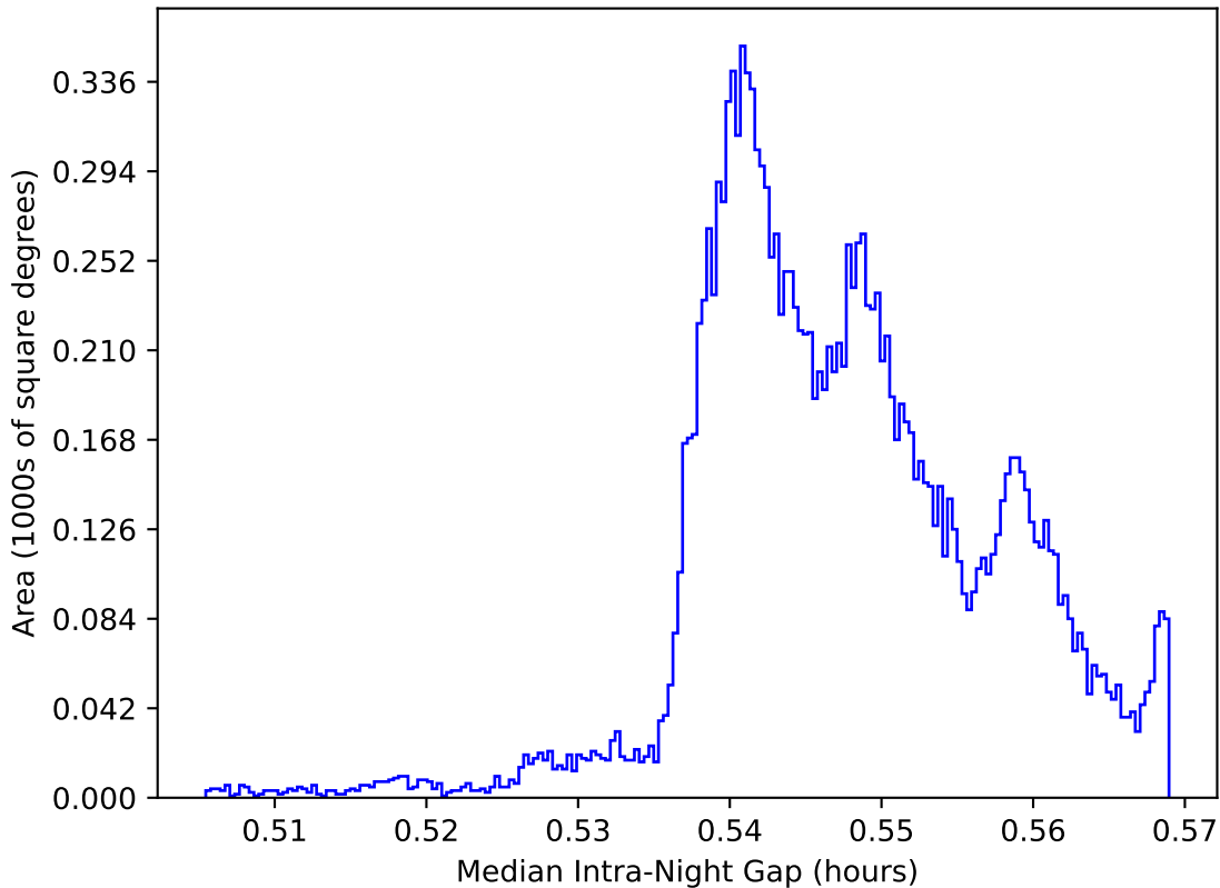
ddf_acor_sf10_ls15_lsr10_v3.4_10yrs WFD: Median Intra-Night Gap
