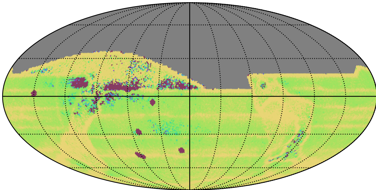
ddf_acor_sf10_lsf15_lsr10_v3.4_10yrs All sky: Median Intra-Night Gap
