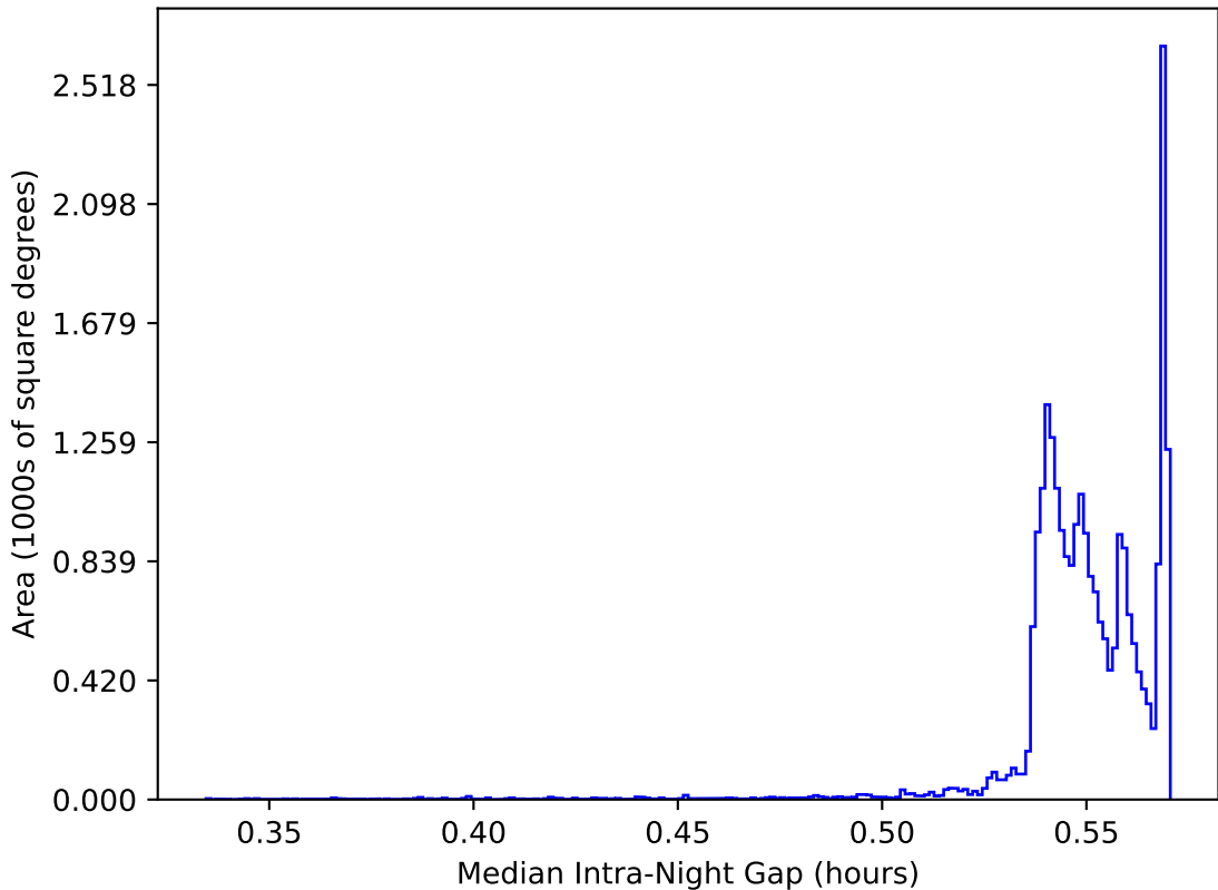
ddf_acor_sf10_lsf15_lsr10_v3.4_10yrs All sky: Median Intra-Night Gap
