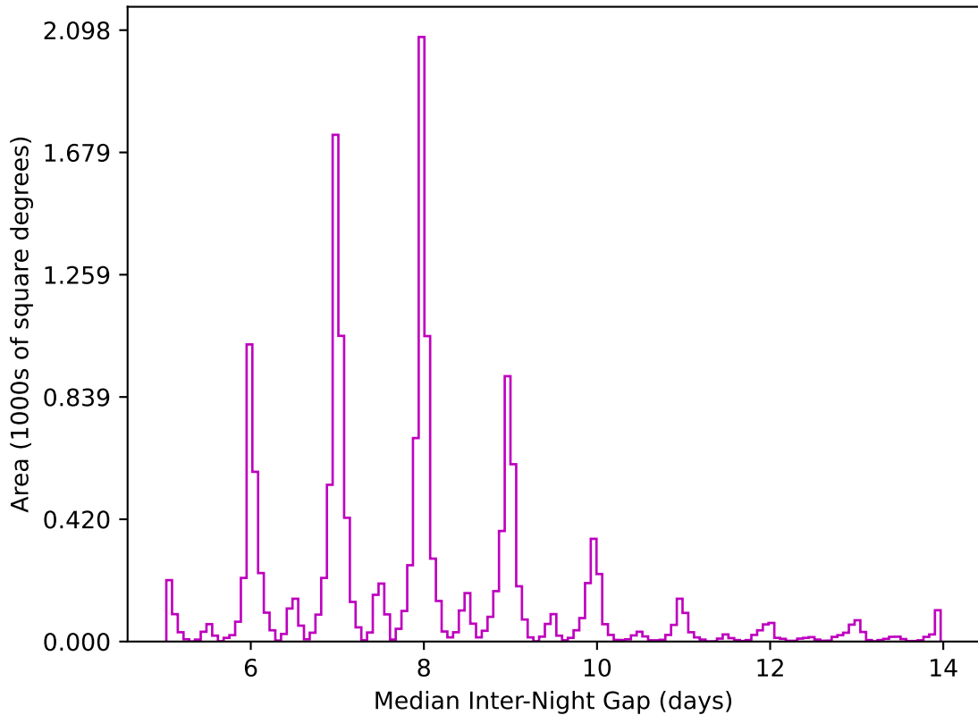
ddf_acor_sf10_lsf15_lsr10_v3.4_10yrs WFD z band: Median Inter-Night Gap
