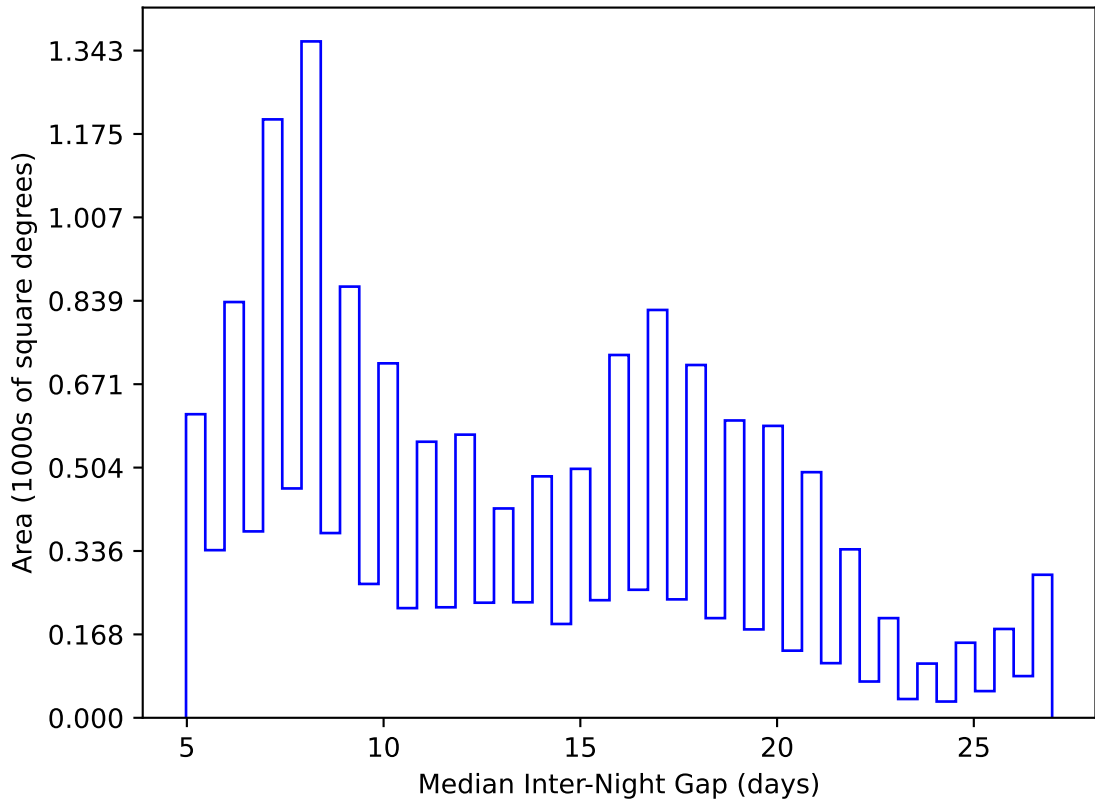
ddf_acor_sf10_lsf15_lsr10_v3.4_10yrs WFD y band: Median Inter-Night Gap
