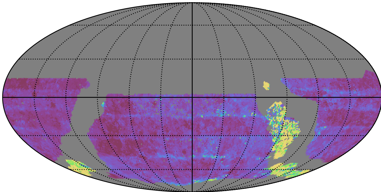
ddf_acor_sf10_lsf15_lsr10_v3.4_10yrs WFD u band: Median Inter-Night Gap
