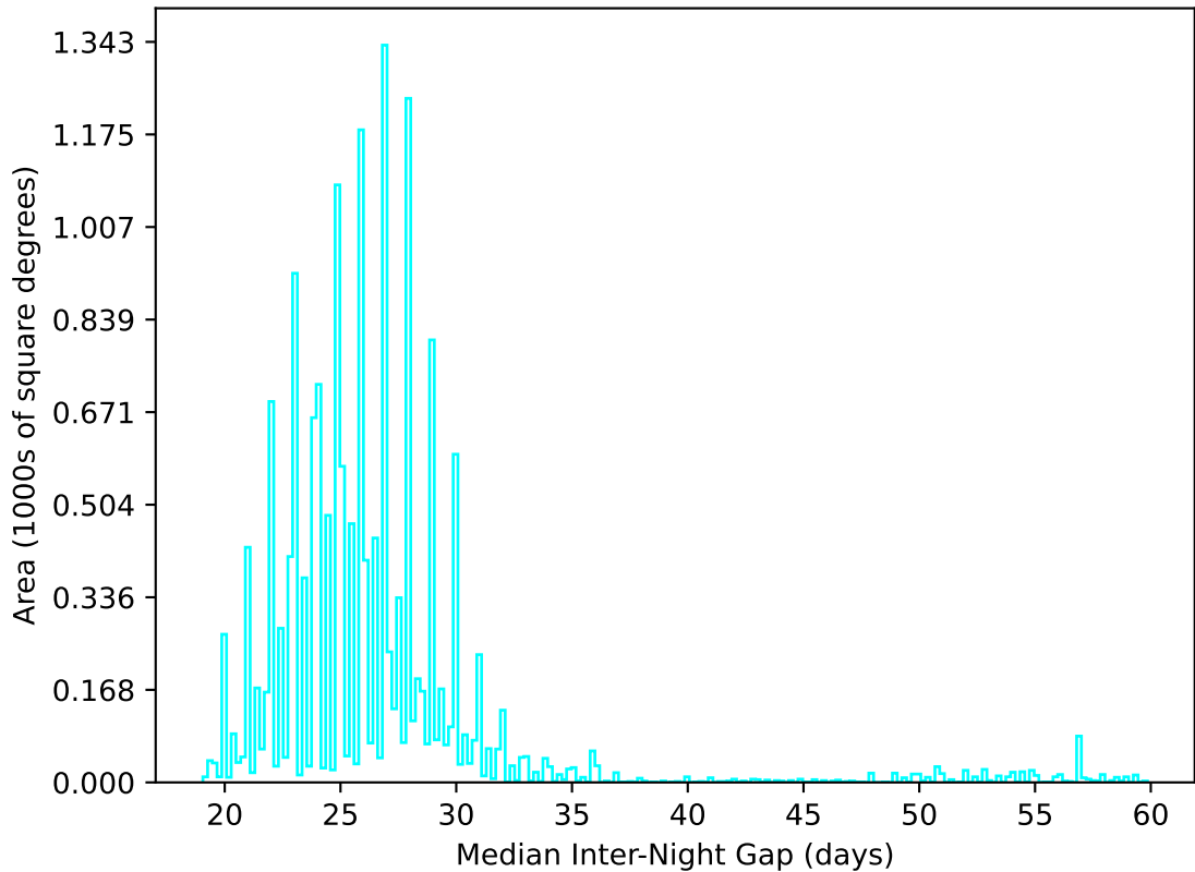
ddf_acor_sf10_lsf15_lsr10_v3.4_10yrs WFD u band: Median Inter-Night Gap
