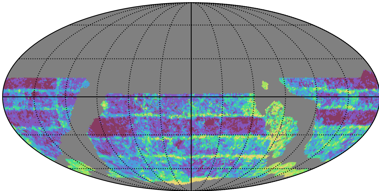
ddf_acor_sf10_lsf15_lsr10_v3.4_10yrs WFD r band: Median Inter-Night Gap
