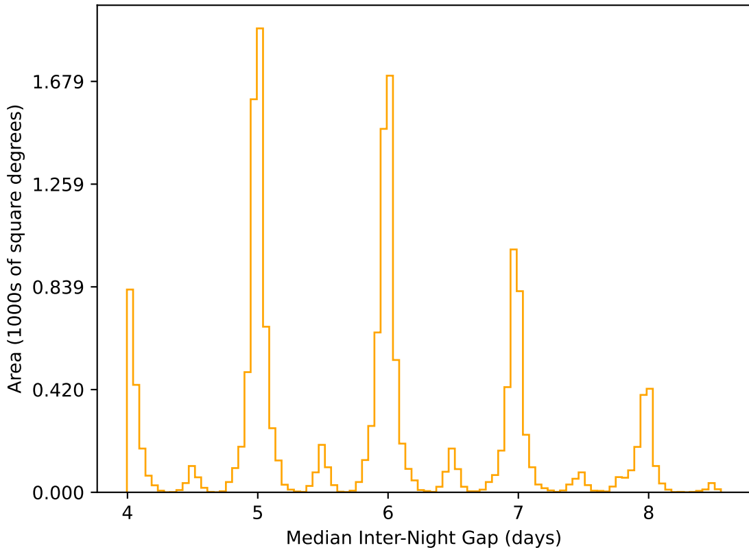
ddf_acor_sf10_lsf15_lsr10_v3.4_10yrs WFD r band: Median Inter-Night Gap
