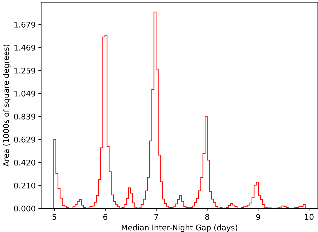
ddf_acor_sf10_ls15_lsr10_v3.4_10yrs WFD i band: Median Inter-Night Gap
