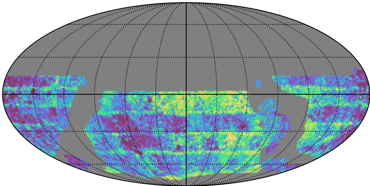
ddf_acor_sf10_lsf15_lsr10_v3.4_10yrs WFD g band: Median Inter-Night Gap
