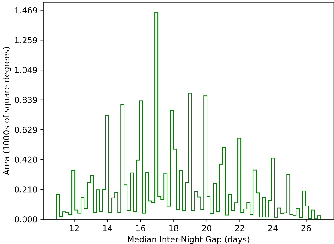
ddf_acor_sf10_lsf15_lsr10_v3.4_10yrs WFD g band: Median Inter-Night Gap
