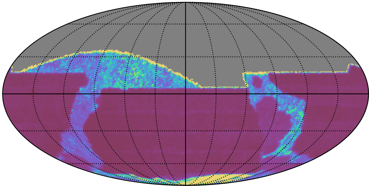
ddf_acor_sf10_lsf15_lsr10_v3.4_10yrs All sky z band: Median Inter-Night Gap
