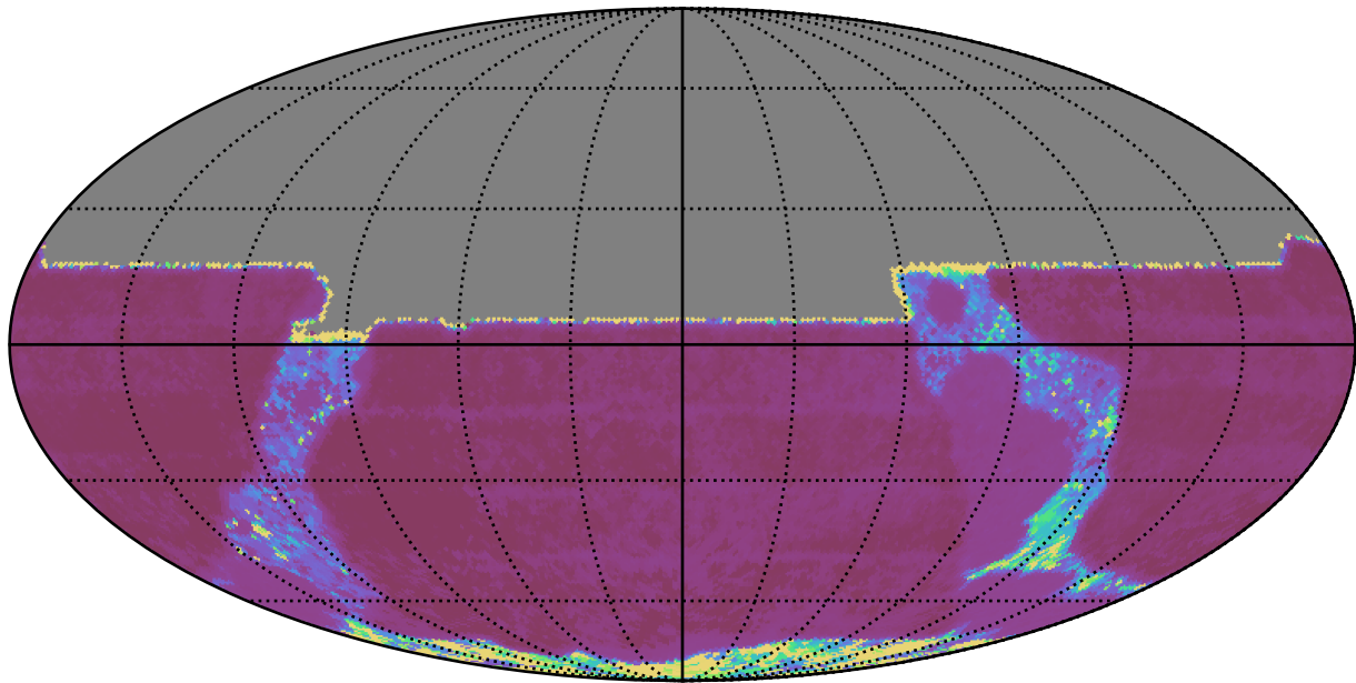
ddf_acor_sf10_lsf15_lsr10_v3.4_10yrs All sky y band: Median Inter-Night Gap
