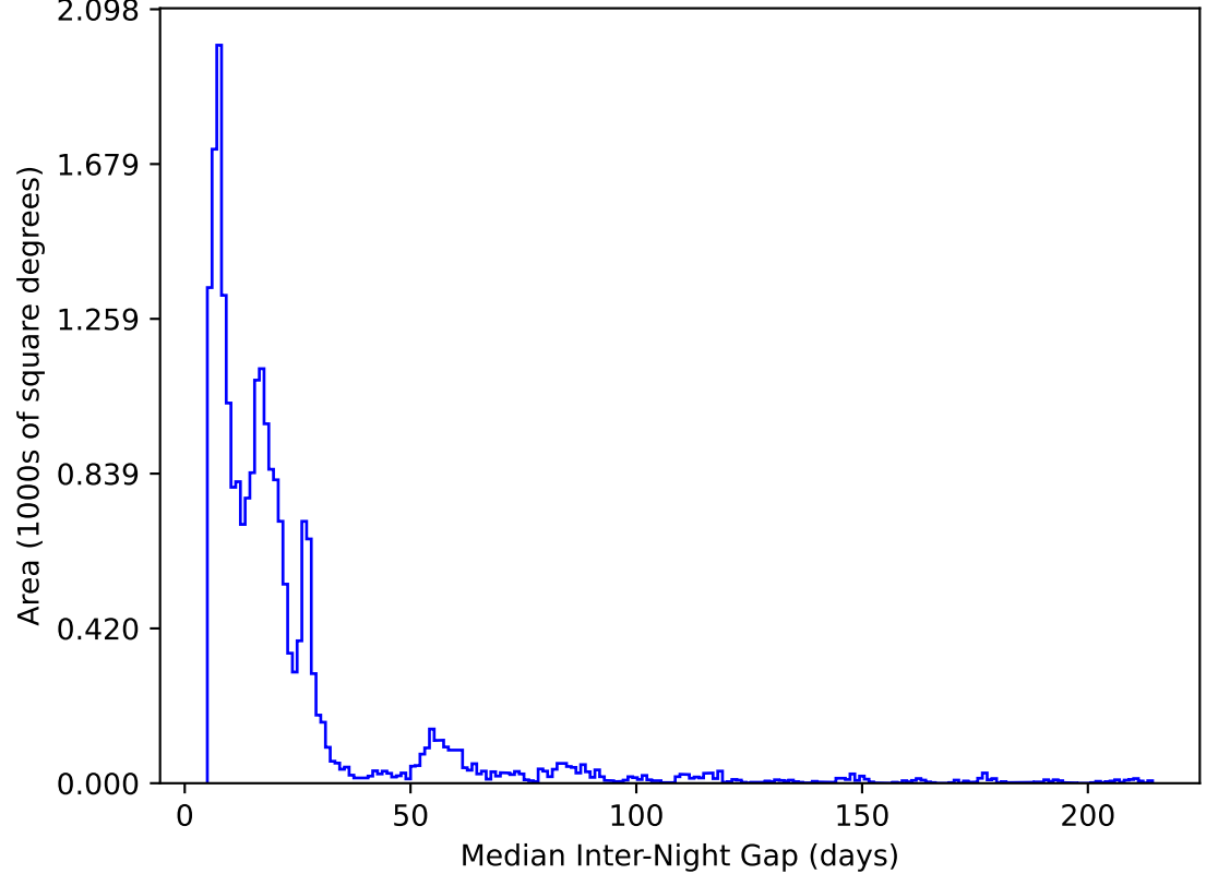
ddf_acor_sf10_lsf15_lsr10_v3.4_10yrs All sky y band: Median Inter-Night Gap
