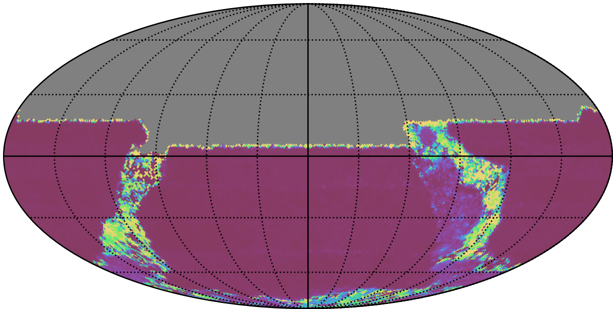
ddf_acor_sf10_lsf15_lsr10_v3.4_10yrs All sky u band: Median Inter-Night Gap
