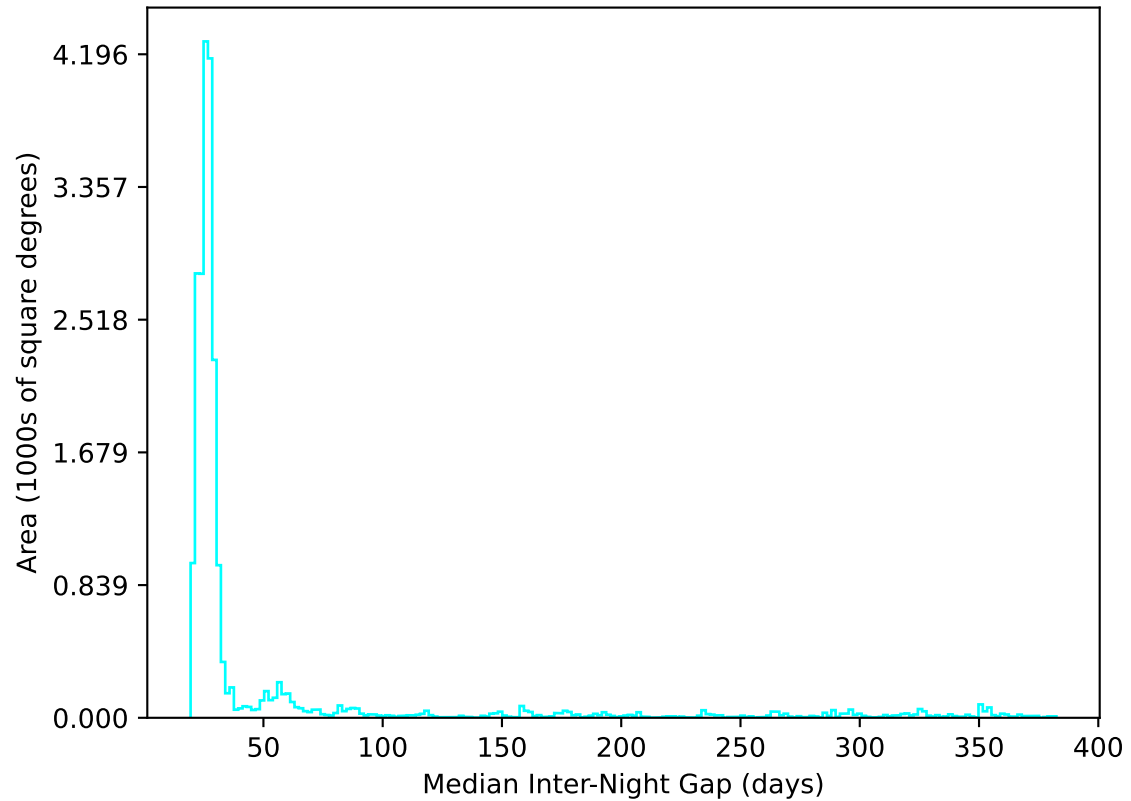
ddf_acor_sf10_lsf15_lsr10_v3.4_10yrs All sky u band: Median Inter-Night Gap
