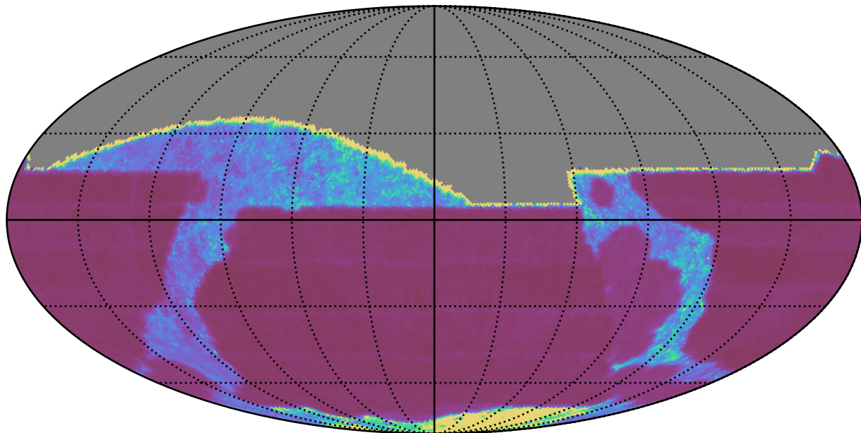
ddf_acor_sf10_lsf15_lsr10_v3.4_10yrs All sky i band: Median Inter-Night Gap
