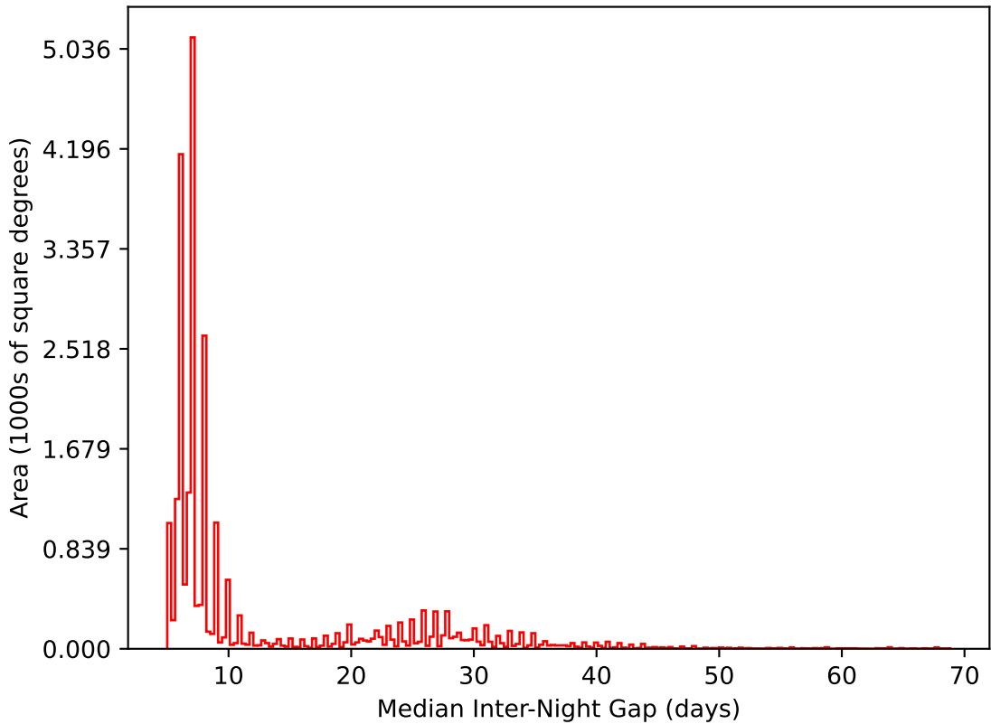
ddf_acor_sf10_lsf15_lsr10_v3.4_10yrs All sky i band: Median Inter-Night Gap
