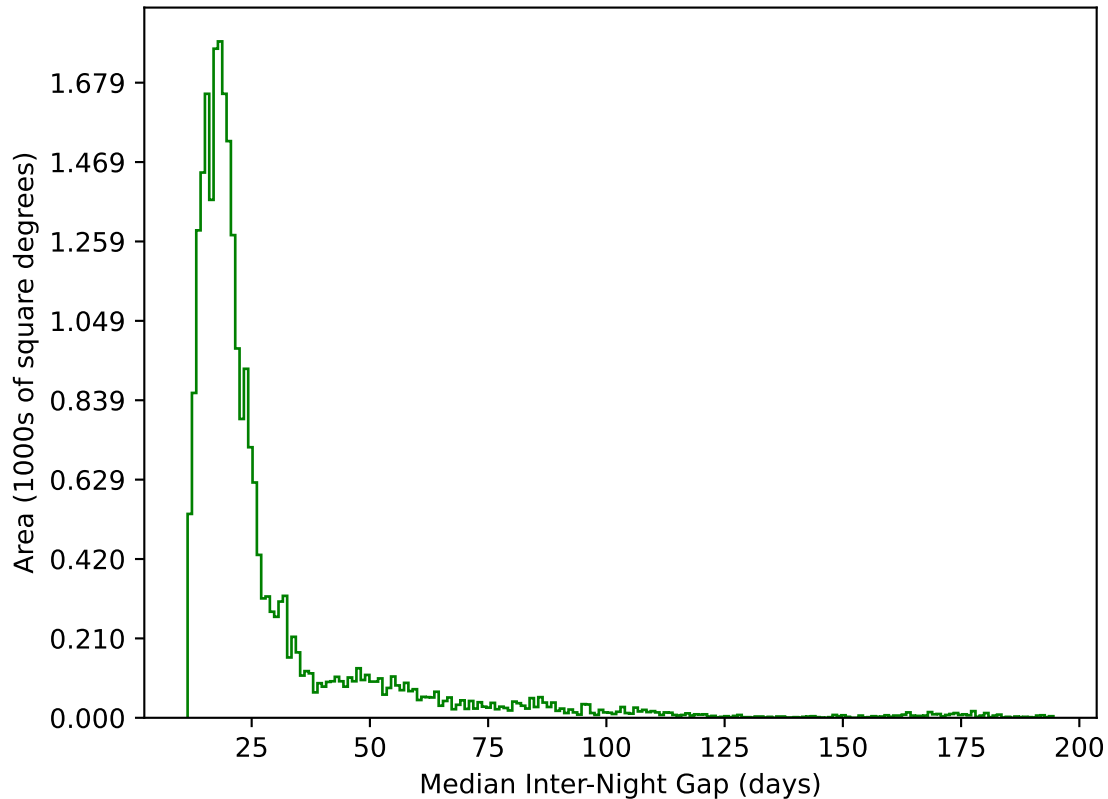
ddf_acor_sf10_lsf15_lsr10_v3.4_10yrs All sky g band: Median Inter-Night Gap
