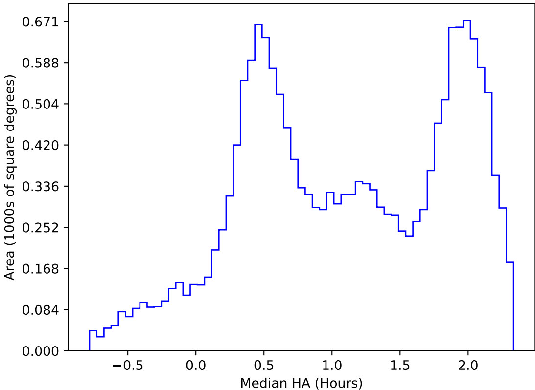
ddf_acor_sf10_lsf15_lsr10_v3.4_10yrs WFD z band: Median HA
