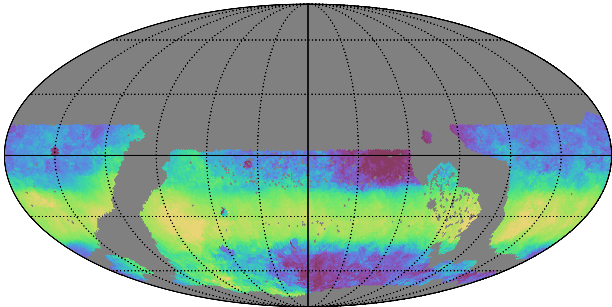
ddf_acor_sf10_lsf15_lsr10_v3.4_10yrs WFD y band: Median HA
