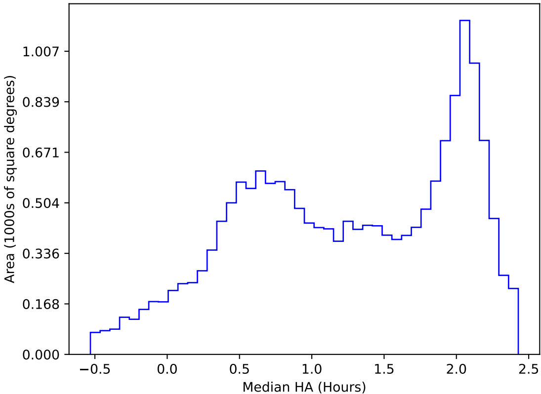
ddf_acor_sf10_lsf15_lsr10_v3.4_10yrs WFD y band: Median HA
