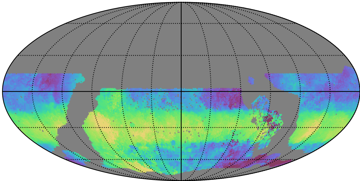
ddf_acor_sf10_lsf15_lsr10_v3.4_10yrs WFD u band: Median HA
