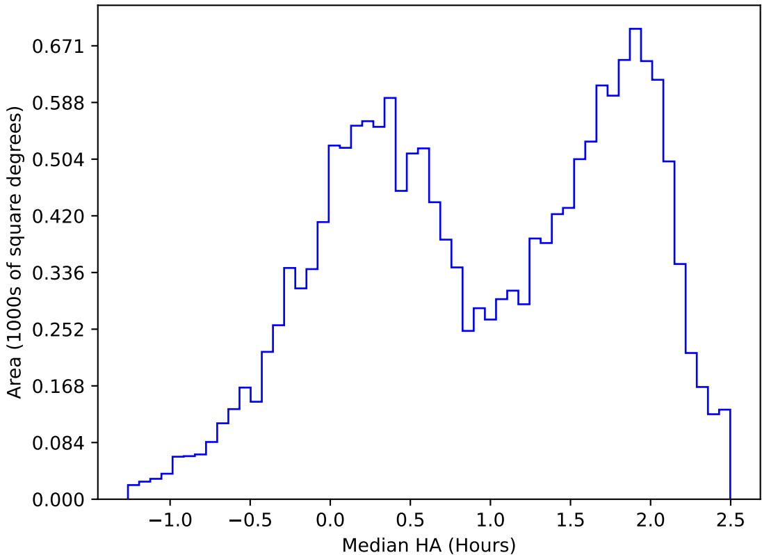
ddf_acor_sf10_lsf15_lsr10_v3.4_10yrs WFD u band: Median HA
