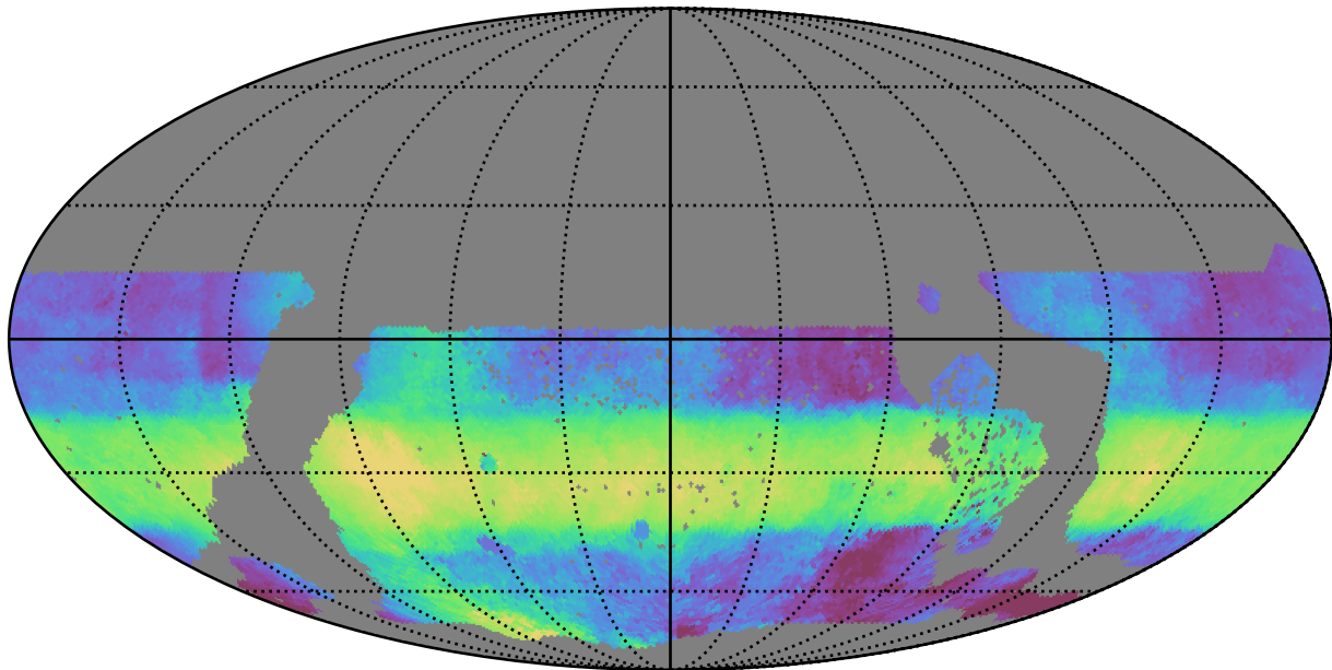
ddf_acor_sf10_lsf15_lsr10_v3.4_10yrs WFD r band: Median HA
