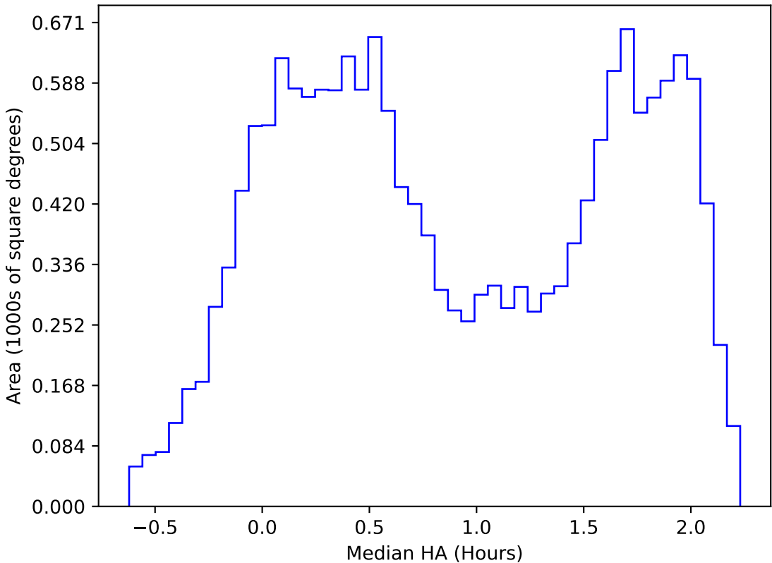
ddf_acor_sf10_lsf15_lsr10_v3.4_10yrs WFD r band: Median HA
