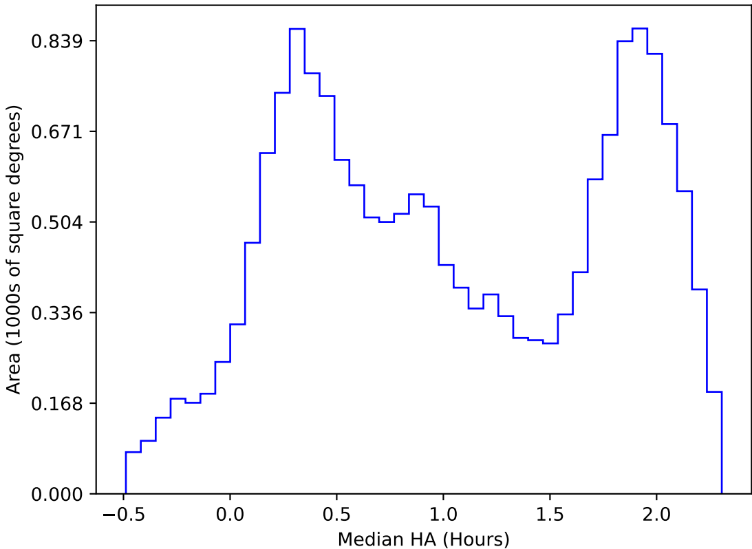
ddf_acor_sf10_lsf15_lsr10_v3.4_10yrs WFD i band: Median HA
