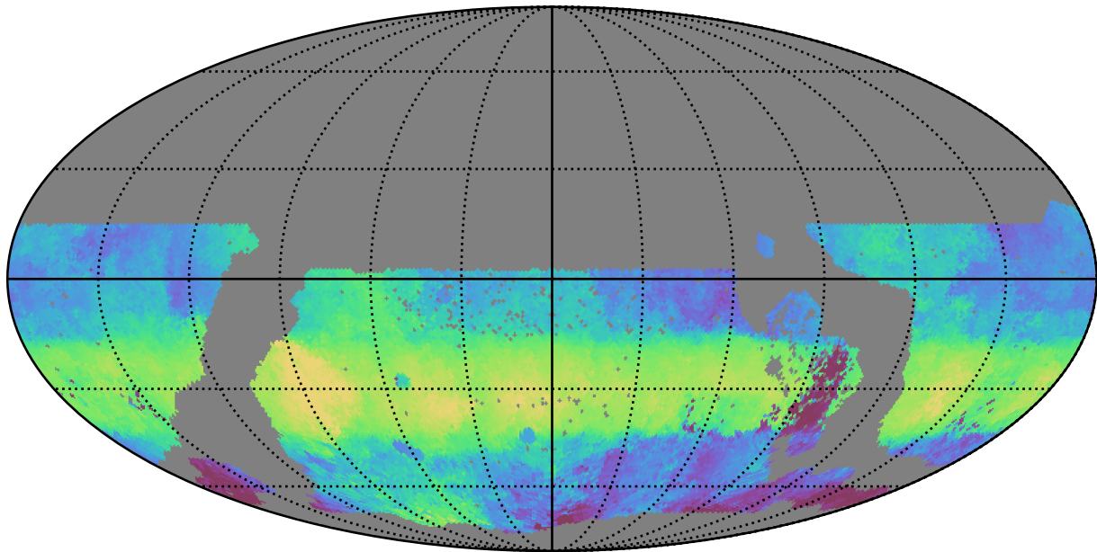
ddf_acor_sf10_lsf15_lsr10_v3.4_10yrs WFD g band: Median HA
