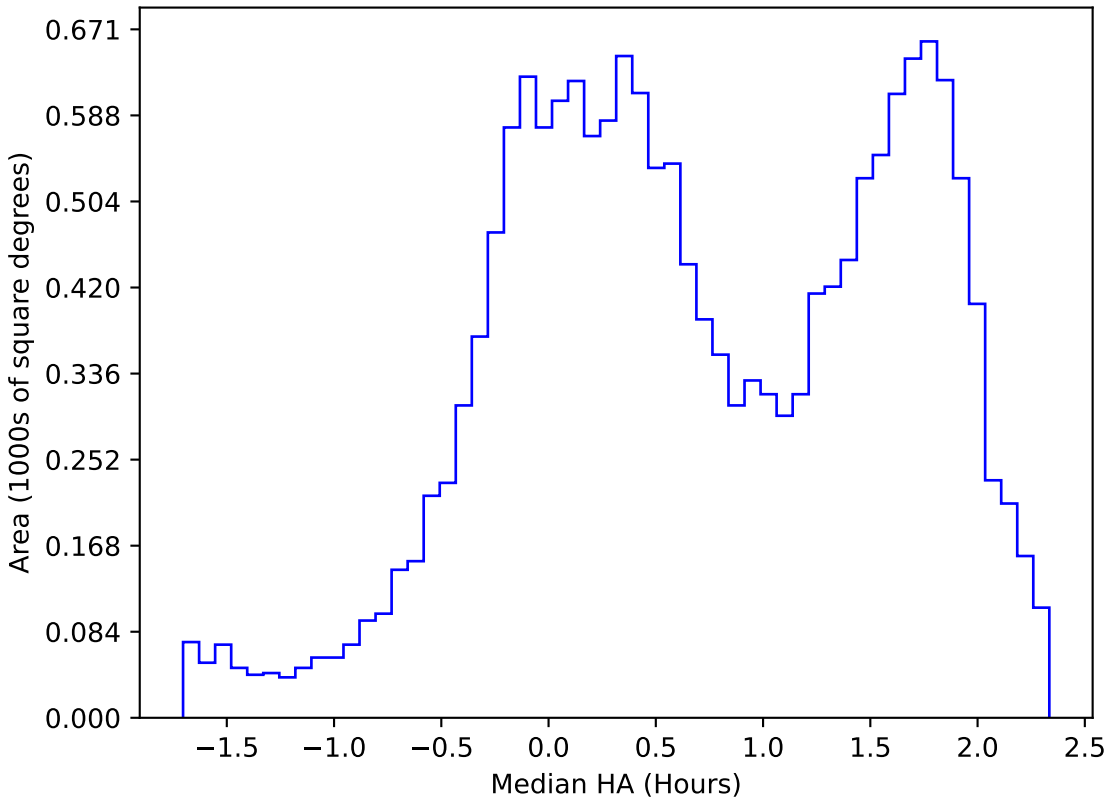
ddf_acor_sf10_lsf15_lsr10_v3.4_10yrs WFD g band: Median HA
