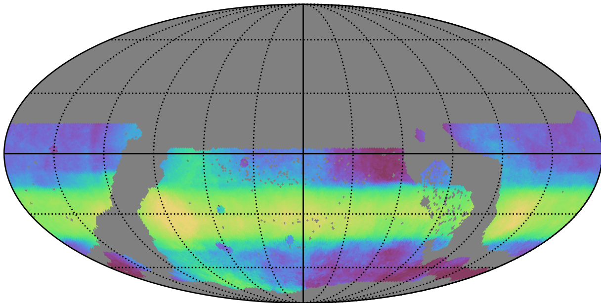
ddf_acor_sf10_lsf15_lsr10_v3.4_10yrs WFD all bands: Median HA
