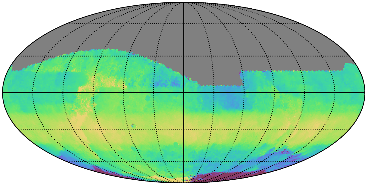
ddf_acor_sf10_lsf15_lsr10_v3.4_10yrs All sky z band: Median HA
