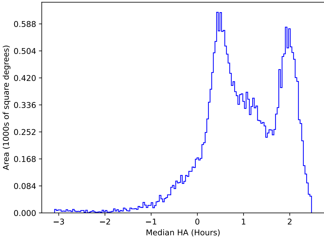
ddf_acor_sf10_lsf15_lsr10_v3.4_10yrs All sky z band: Median HA
