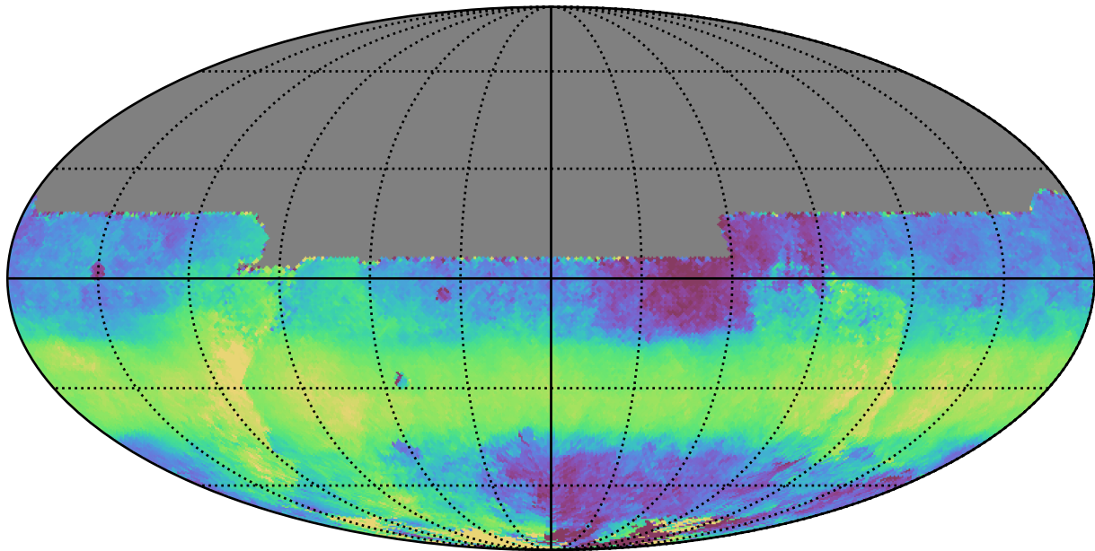
ddf_acor_sf10_lsf15_lsr10_v3.4_10yrs All sky y band: Median HA
