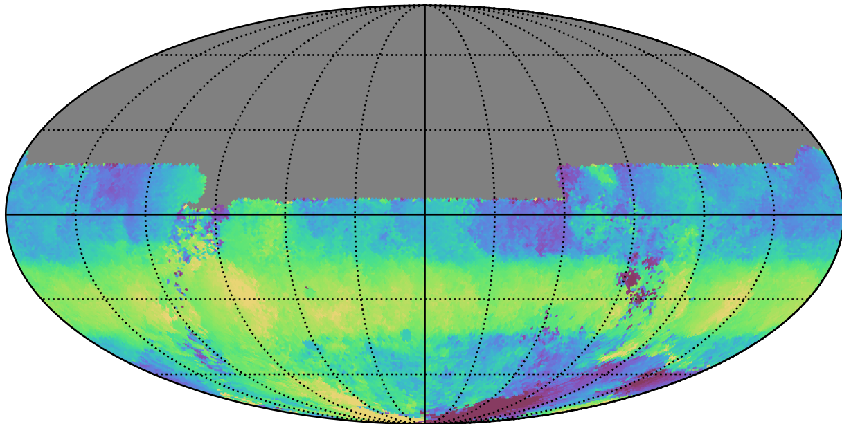
ddf_acor_sf10_lsf15_lsr10_v3.4_10yrs All sky u band: Median HA
