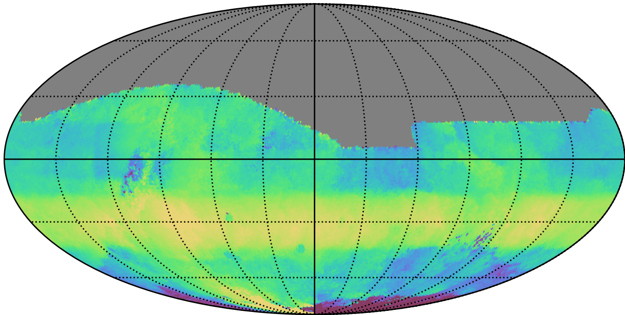
ddf_acor_sf10_lsf15_lsr10_v3.4_10yrs All sky r band: Median HA
