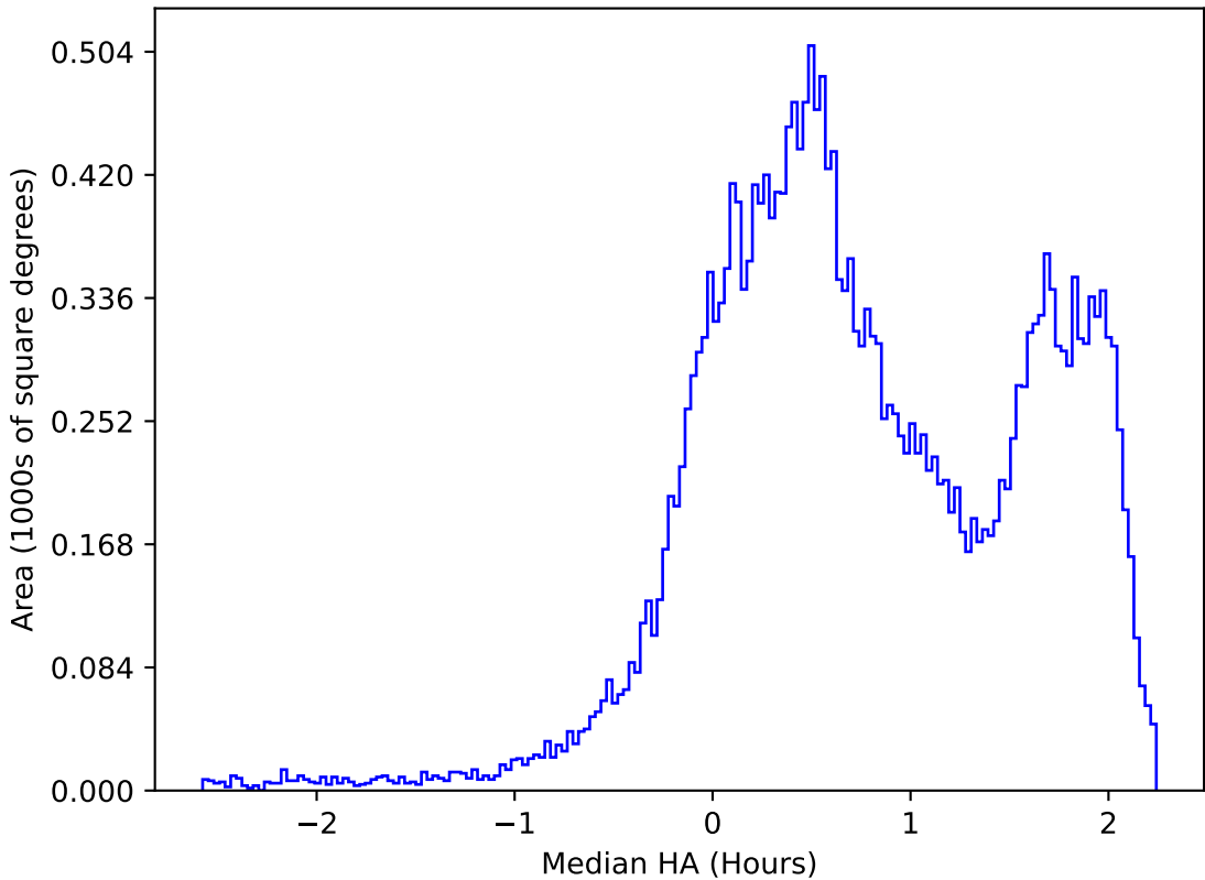
ddf_acor_sf10_lsf15_lsr10_v3.4_10yrs All sky r band: Median HA
