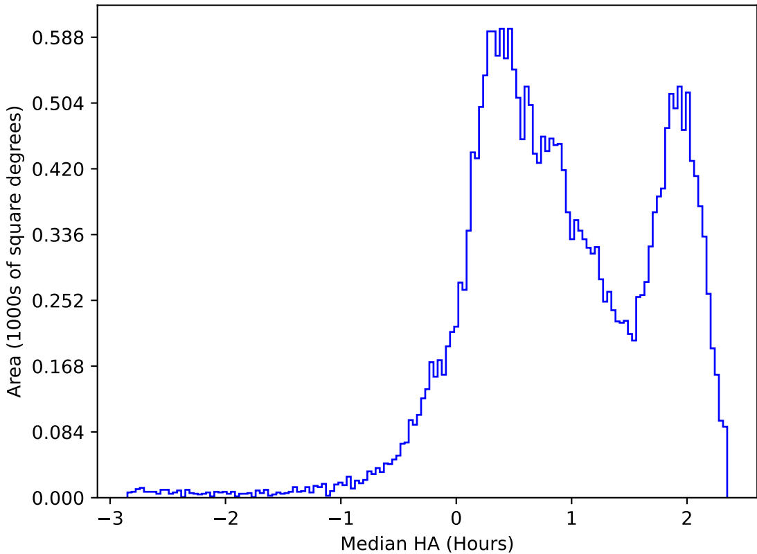
ddf_acor_sf10_lsf15_lsr10_v3.4_10yrs All sky i band: Median HA
